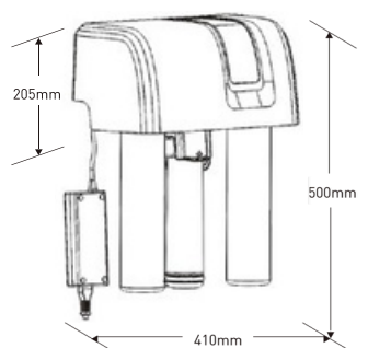
Everpure RO-200U Reverse Osmosis System
